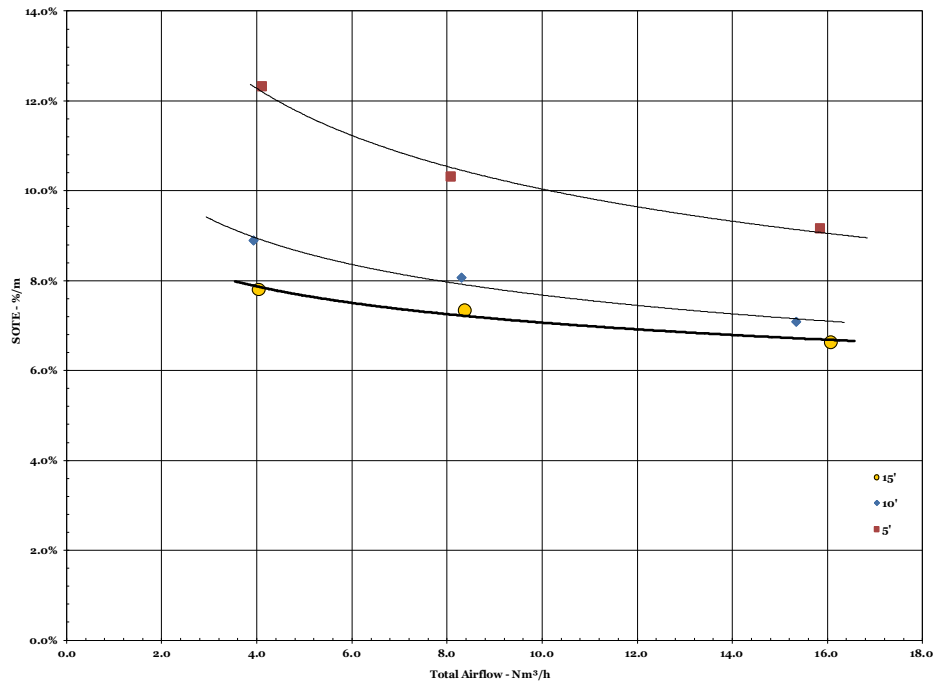
Figure 5-5 SCFM/100' of tubing v. SOTE - 1/2" Bubble Tubing™
